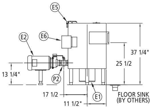
SP-50S (W/ 9" TANGENTIAL TROUGH ADAPTER) MULTIPLE REMOTE ELEVATION VIEW
