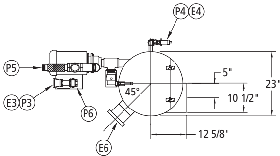
SP-50S (W/ 9" TANGENTIAL TROUGH ADAPTER) MULTIPLE REMOTE ELEVATION VIEW
