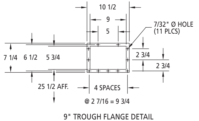
PULPER TROUGH DETAIL
