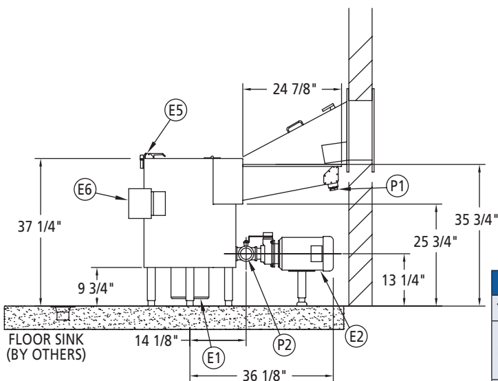
SP-50S (W/ TRAY FEED ADAPTER) OPTIONAL PASS THRU WINDOW ELEVATION VIEW
