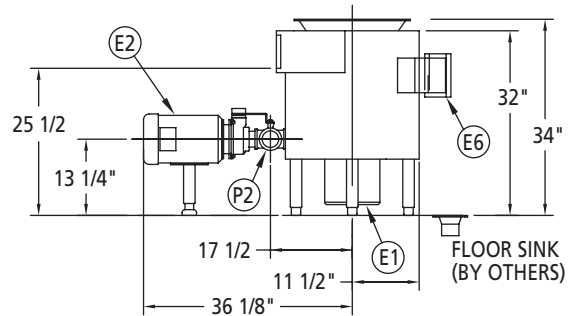
TYPICAL ELEVATION VIEW SP-50 UDT PULPER
