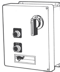
RAC2 Control Center Automatic Reversing
